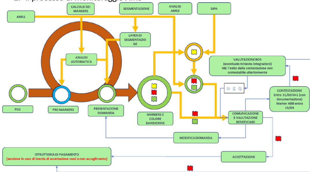
FIGURA 1 WORKFLOW AMS
